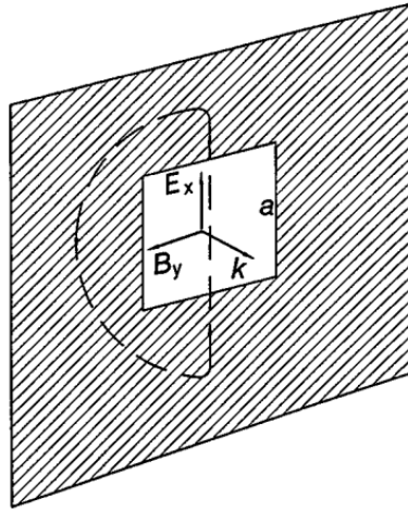
Figure 2: A screen with a square aperture of side a is illuminated by a linearly polarized electromagnetic wave. The imaginary loop shown by the dashed curve lies close to the screen, on the side away from the source, and so is partly in the shadow of the wave.
