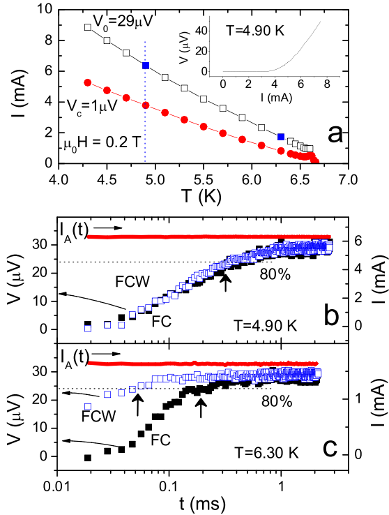
FIG. 1 (color online). (a) Temperature dependence of critical current defined by a 1 \mu\text{V} criterion (solid circles) showing the peak effect at 6.60 K. Open squares: current values corresponding to a saturation voltage V_0 = 29 \mu\text{V} . Inset: V-I curve obtained with slow current ramp. The two solid squares mark the levels of the current pulses in (b) and (c). (b) Onset of motion as monitored by evolution of the voltage response to a current pulse of fixed amplitude I_A = 6.3 mA (solid line) at 4.90 K for V_0 = 29 \mu\text{V} . Solid squares, FC state; open squares, FCW state. (c) Same as (b) at 6.30 K. Note that here I_A = 1.63 mA. Vertical arrows show the definition of \tau_{80} .
