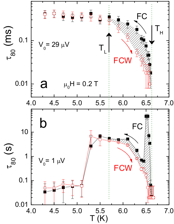
FIG. 2 (color online). (a) Temperature dependence of \tau_{80} at V_0 = 29 \mu\text{V} for FC and FCW states showing the position of T_L and of T_H . (b) Temperature dependence of \tau_{80} at V_0 = 1 \mu\text{V} . The position of T_L and T_H is the same as in (a).
