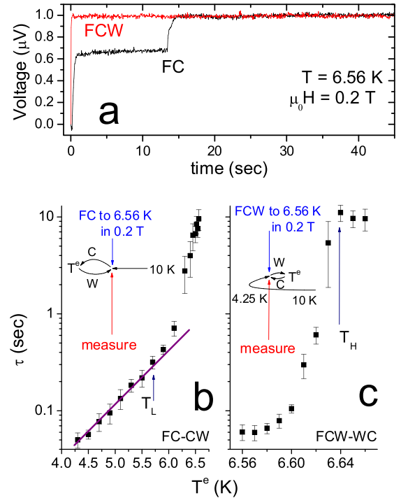
FIG. 3 (color online). (a) Time evolution of response to current pulse measured at T^m = 6.56 \text{ K} and V_0 = 1 \mu\text{V} for FC and FCW lattices. (b) Response times for FC-CW lattices as a function of preparation temperature T^e , illustrating the definition of T_L . The preparation sequence, described in the text, is schematically sketched. The solid line represents a fit to the data as discussed in the text. (c) Response times for FCW-WC, illustrating the definition of T_H .
