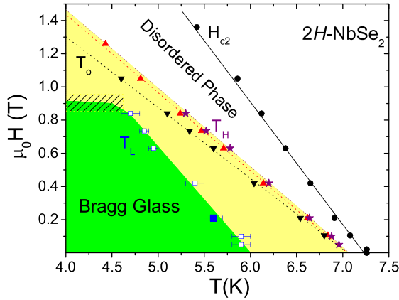
FIG. 4 (color online). H - T phase diagram showing the line T_L (squares), below which topological defects become scarce, and T_H (stars) the limit of superheating of the Bragg glass. Also shown are T_o (inverted triangles) and T_p (triangle), representing the onset and peak of the peak effect. No data is available for the hashed area.
