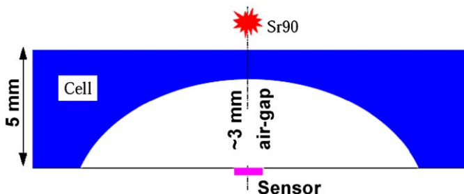
Fig. 4. Concave tile uniformity scan schematic (not to scale).
