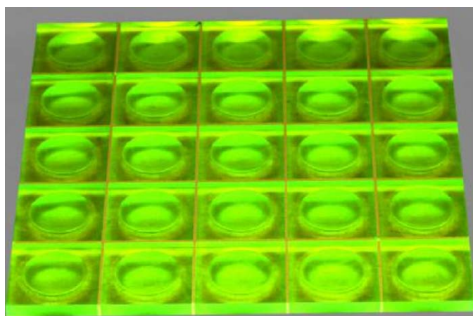
Fig. 11. Array (mega-tile) of 5 mm thick, 9 cm 2 concave square tiles with two alignment holes.
