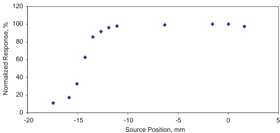
Fig. 5. Response uniformity for a square concave tile.
