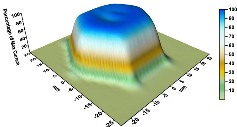
Fig. 7. Response uniformity for a hexagonal concave tile.
