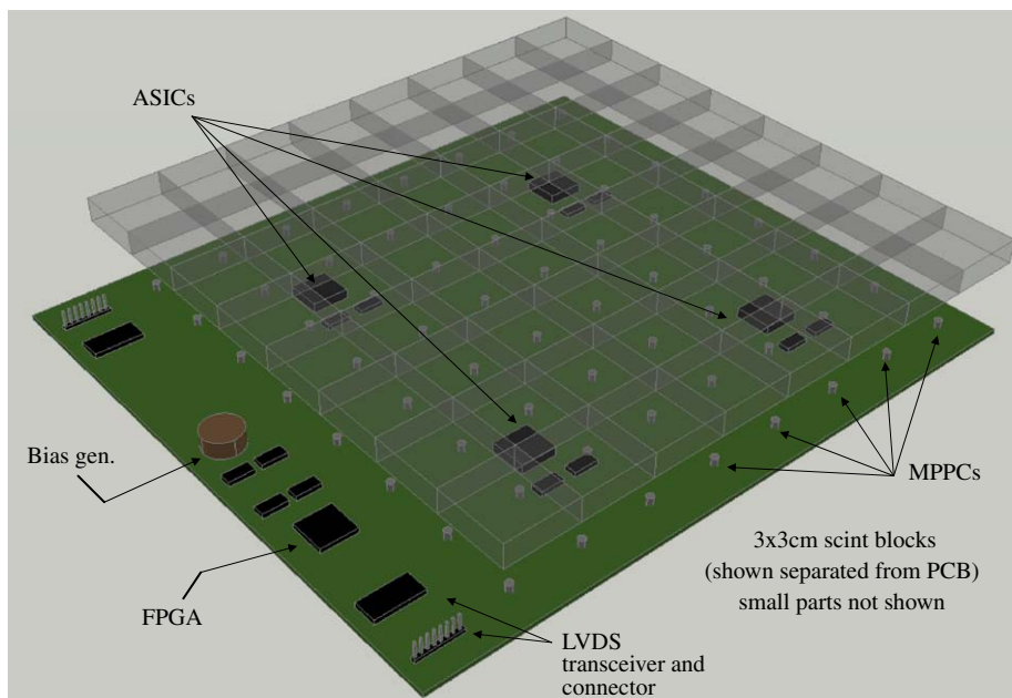
Fig. 10. Integrated readout layer concept.
