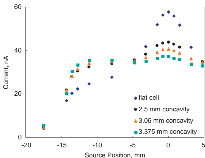
Fig. 8. Response uniformity of a square tile with different depths of concavity.
