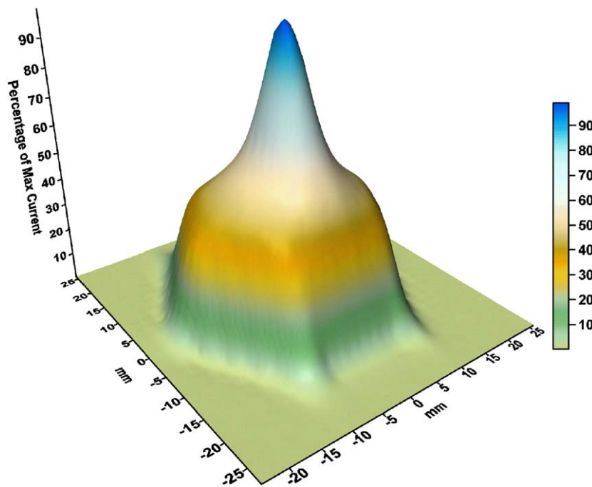
Fig. 6. Response uniformity for a hexagonal flat tile.
