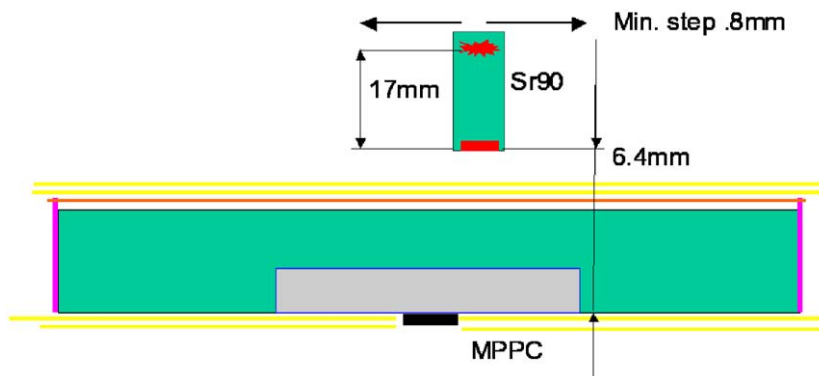
Fig. 1. Tile uniformity scan schematic (not to scale).
