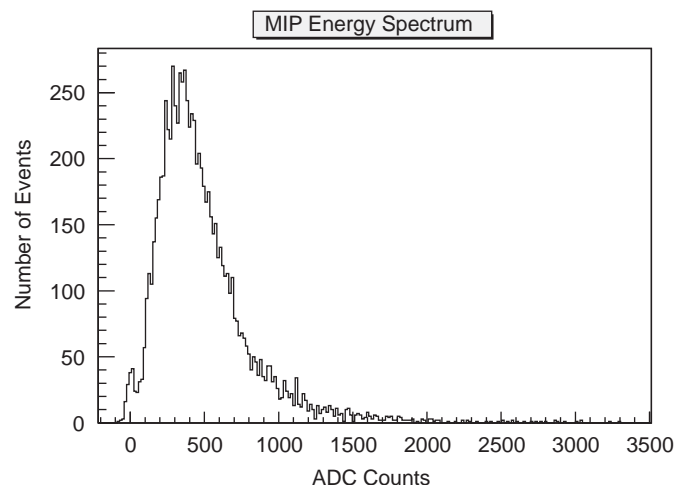
Fig. 9. Response of a directly coupled concave tile to cosmic ray muons.
