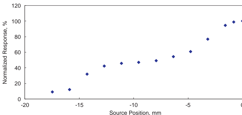
Fig. 2. Response uniformity for a square flat tile as a function of the distance from its center where the sensor is located.
