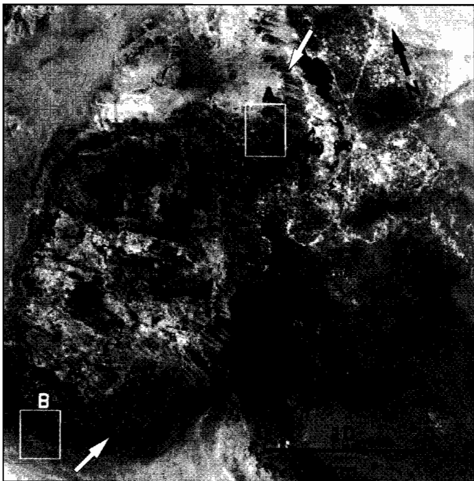
Figure 11. SPOT panchromatic image covering the Farafra study area. The oval-shaped body in the western portion of the image is El Quss Abu Said Plateau. The plateau is composed of mostly limestone of Farafra Formation. The areas with dark albedo in the southwestern corner of the plateau are sandstones of Mingqar El-Talh Formation. White arrows delineate the eastern escarpment, along which a series of pediments and alluvial fans can be identified. Details of areas A and B are shown in Figures 12 and 13, respectively. To the east of the escarpment is the Farafra depression. The black patches in the north-eastern part of the scene are playa deposits. SPOT scene id = (11062961993070909083401P)
