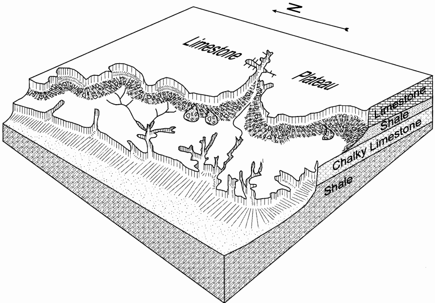
Figure 9. Block diagram of El Rufuf Pass area showing major geomorphic features. A major scalloped escarpment formed in the limestone plateau by differential erosion and ground-water sapping. The slumping blocks developed within the scallops and were disintegrated by weathering and transported downhill by surface runoff. Emerging ground water from the permeable limestone and chalky limestone units formed stubby-looking channels by headward erosion, sapping, and slumping in these units. On the impermeable shale units at the base of the escarpment, surface runoff formed pediments and alluvial fan systems. The lowest shale units formed the depression covered with aeolian sands.
