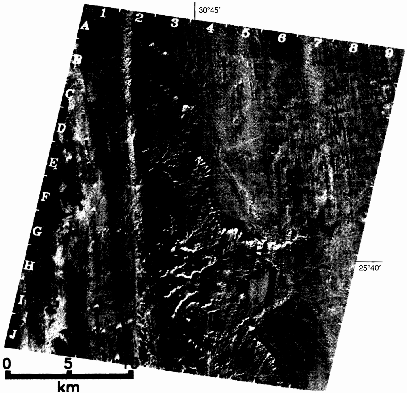
Figure 6. Image of El Rufuf Pass study area constructed by using Thematic Mapper (TM) bands 1, 4, and 7 to provide hue and saturation and SPOT multispectral band 3 to provide intensity, geometrically corrected to compare with geologic map in Figure 2. Sand dunes and wind streaks are visible from coordinates 1–3 and A–J. Areas shown as green (G1–2, J2–3) correspond to vegetation in the Kharga Oasis. Stubby channels are seen in the Tarawan Formation (C3, E3–4, G to I and 4 to 6) and are roughly oriented in north-south, northeast-southwest, east-west directions. Fluvial pediment and alluvial fan systems exist on the Esna Formation to the east of Tarawan Formation (e.g., E to F and 4 to 5, I to J and 7 to 8). The high escarpment is located from A–2 to J–8 and delineates the boundary between the Esna and El Rufuf formations. The escarpment extends into the plateau along a major fault at El Rufuf Pass area (F to G and 7 to 8). Note the scalloped nature of the high escarpment (B3, C to D and 3 to 4). The lack of drainage on the El Rufuf Formation is consistent with high intrinsic permeability associated with karstification. SPOT scene id = (11132981988111908311101X).
