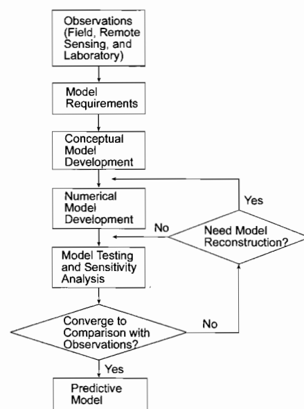
Figure 2. Flow diagram of the modeling approach of this study. The parameter values are selected based on independent measurements documented in the literature if possible. The model was used to estimate the few parameters that have no independent constraint by comparing model outputs with the observations. The result is a predictive model that can provide insights into processes that are no longer operating.
