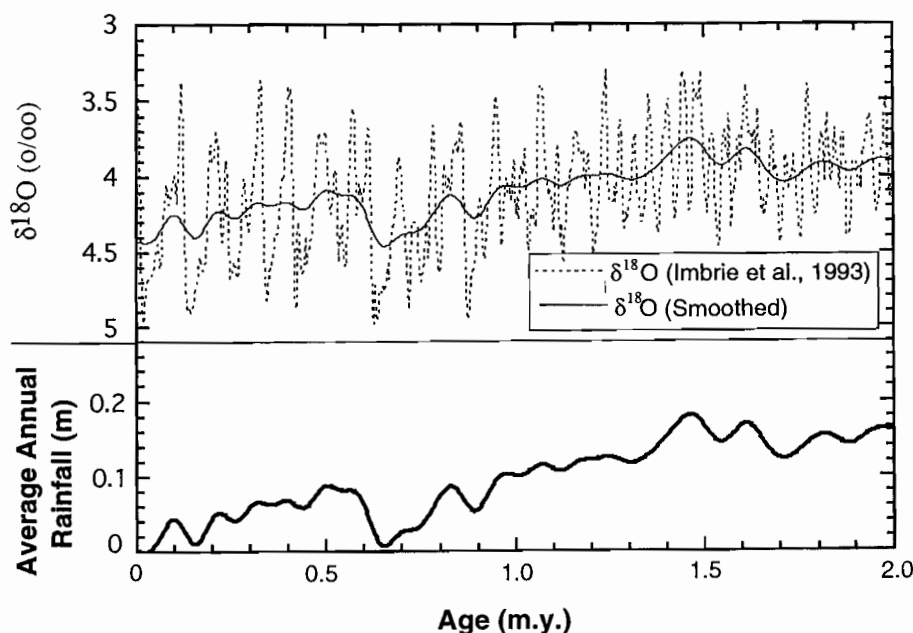
Figure 16. Average annual rainfall function (bottom) as defined from the composite deep-sea core \delta^{18}\text{O} record (top, Imbrie et al., 1993). Also shown in top panel is the smoothed version of the \delta^{18}\text{O} record, which is used to scale the changing climate rainfall function. The smoothed version was obtained by taking a three-point average of the original data consecutively for 200 times.
