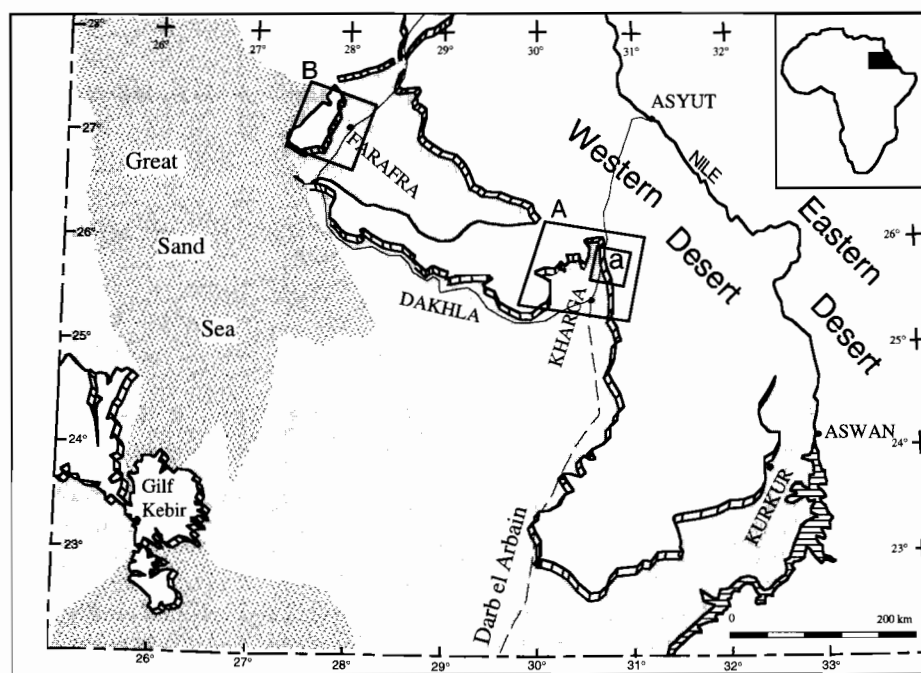
Figure 1. Location map of Western Desert, Egypt, showing major depressions (dark stipple areas), plateaus, and aeolian sand deposits. Escarpments bordering the depressions extend for hundreds of kilometers. Box a denotes the study area shown in Figures 3 and 6. Boxes A and B denote footprints of Thematic Mapper data and Système Probatoire d'Observation de la Terre (SPOT) data shown in Figures 5 and 11, respectively. Study areas visited in the field include the Kharga, Farafra, and Kurkur regions (adapted from Hermina, 1990).
