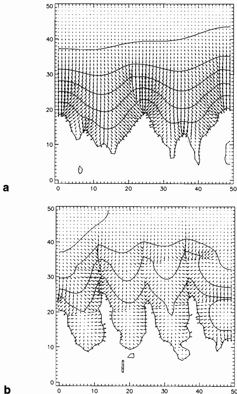
Figure 18. Ground-water flowlines and contours at 0.8 m.y. in time. The grid is resampled to half resolution for clarity (otherwise arrows clutter together) and only the active ground-water cells of the grid are shown. The numbers along x and y axes identify the columns and rows of the resampled grid. (Each dimension is 17 km.) The outcrop of the original contact boundary between limestone and shale is along the x axis of the figure. The areas filled with arrows are limestone and the white areas are exposed shales. (a) With no fractures. Ground-water flowlines converge toward the scallop depressions and diverge away from the ridges between scallops. (b) With fractures. Flowlines not only converge toward scalloped depressions, but also concentrate toward the fracture zones.
