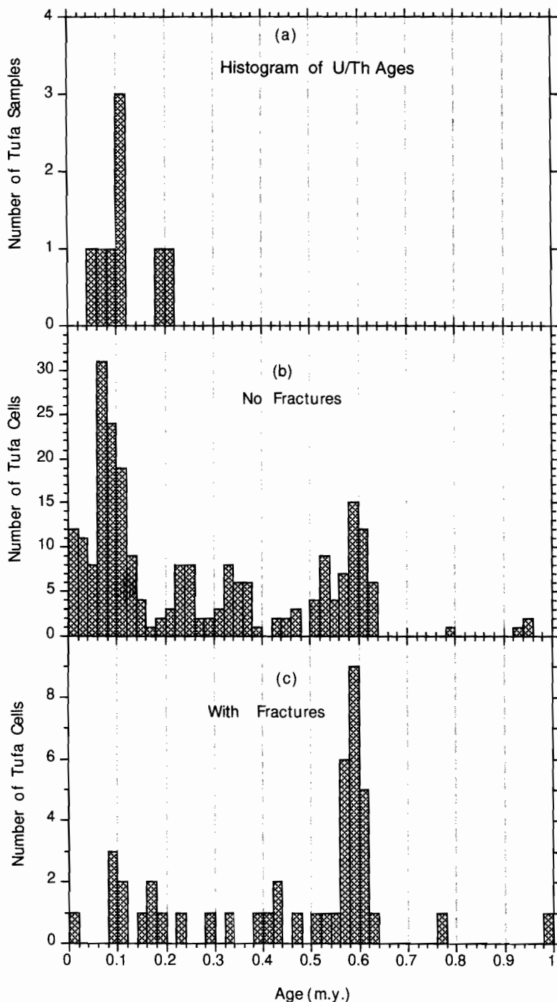
Figure 19. U/Th ages of tufas from the Farafra (1 sample) and Kurkur (7 samples) areas are shown in histogram (a). Model tufa age histograms for \delta^{18}\text{O} -forced changing climate (b and c) are aligned vertically for comparison. The \delta^{18}\text{O} -forced models (b and c) produced tufa ages consistent with U/Th ages. Note that the scales of the y axes are different. U/Th data from Sultan et al. (1996) and Crombie et al. (1995, 1997).
