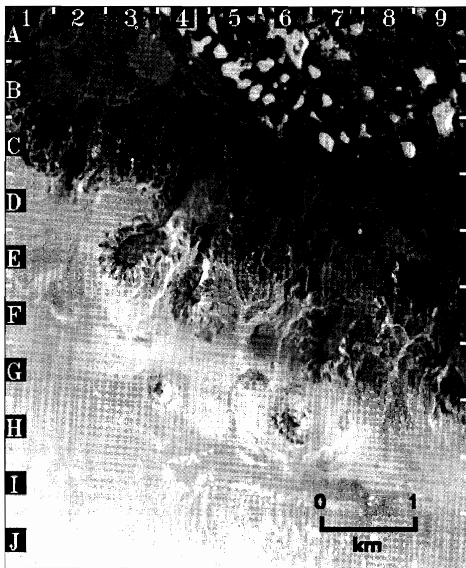
Figure 13. Enlargement of box B in Figure 11. The escarpment extends from B1 to G9. To the north of the escarpment is the plateau, composed of sandstone of the Minqar El-Talh Formation. To the south is the depression underlain by the Esna (shales) and Tarawan formations (chalks). The scallops along the escarpment (E to F and 3 to 4, E to G and 7) are more elongated and more irregular compared to those shown in Figure 10. The ridges between the scallops are also wider and isolated inselbergs are left in the depression (G to H and 3 to 4, H6).
