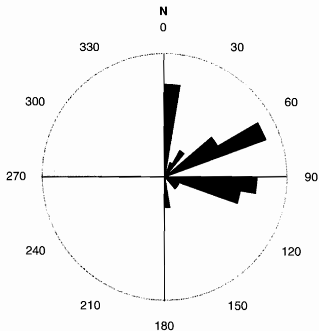
Figure 8. Rose diagram of the trends of channels in the Tarawan Formation and El-Rufuf Formation, measured from SPOT and Thematic Mapper data (i.e., Fig. 6). The major trends are in the north-south, northeast-southwest, and east-west, generally consistent with structural trends of this area documented in the literature (e.g., Hermina, 1990; Said, 1962).
