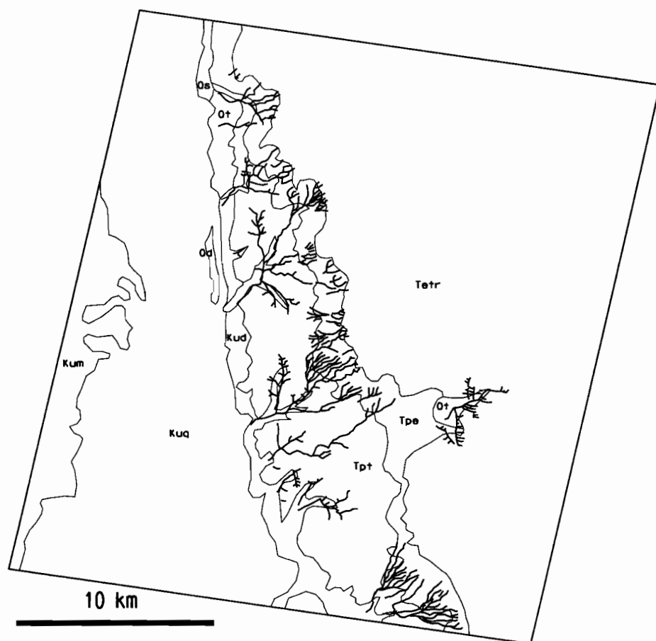
Figure 7. Drainage patterns of the El Rufuf Pass area superimposed with geologic boundaries. See Figure 3 caption for formation names. Thin lines show the geologic boundaries and the thick lines show the drainage systems. The drainage density in the shale unit (Tpe) is high compared with those in the carbonates units (Tetr and Tpt). The tributaries enter the main streams at high angles in the carbonate units, whereas those in the shale form a parallel pattern. The drainage system is constructed from the satellite data (Fig. 6) using a Geographic Information System software (MGE by Intergraph Corporation).
