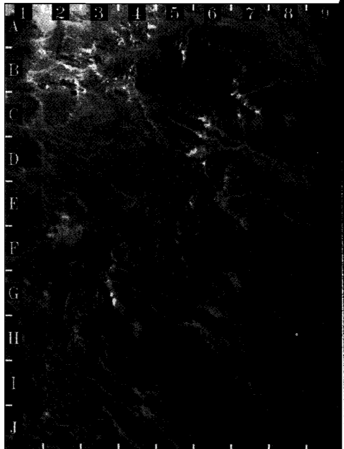
Figure 12. Enlargement of box A in Figure 11. The escarpment extends from coordinates J-1 to B-7. To the west of this line is the limestone plateau and to the east is the depression underlain by Dakhla Formation (shales) and Khoman Formation (chalks). No drainage system is evident on the plateau, but there are channels emanating from the base of the escarpment and draining into the depression. The scallop-shaped features along the edge of the escarpment are located at coordinates F to G and 3 to 4. Also note the linear ridges trending north-west-southeast between adjacent scallops (H to G and 3 to 4, E6-7).
