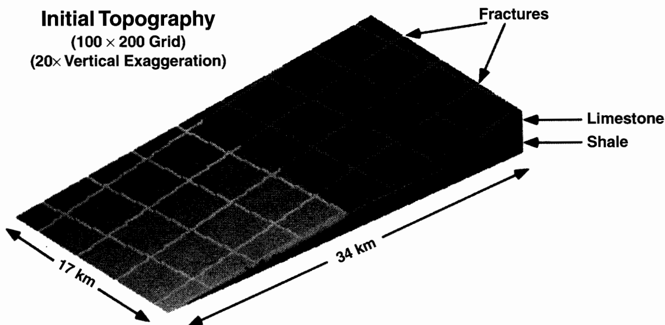
Figure 15. Initial topography and stratigraphy. The slope of the topography surface is 1% (thus Dupuit assumption is valid). The pink is limestone and the bluish-green is shale. Bright lines are high hydraulic conductivity and erodibility zones to simulate fractures (in the shale layer, the bright zones only represent high erodibility). The two layers are assumed to be horizontal. Ground-water flow only operates in the limestone layer.
