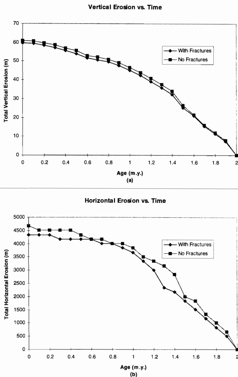
Figure 17. (a) Vertical surface erosion vs. time. (b) Horizontal scarp retreat vs. time. The erosion and retreat are calculated at the outcrop of the boundary between limestone and shale. The slopes of the lines are rates of erosion or retreat. Note the decrease in rates in both cases. Present is 0 m.y.
