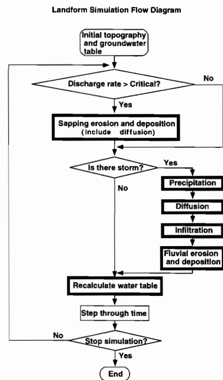
Figure 14. Flow diagram of the computer simulation illustrating erosion, deposition, and ground-water sapping processes and their interactions. See text for details.
