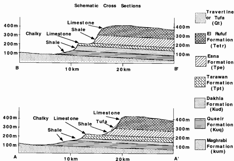
Figure 4. Schematic cross sections along lines AA' and BB' in Figure 2. Note the steep escarpment slopes for the limestone (Tetr) and chalky limestone (Tpt) units and the fact that both are underlain by shales (Kud, Tpe). The tufa deposits on limestone bedrock are spring derived. Topographic information from Joint Operations Graphic, 1:250,000, El-Kharga sheet, Defense Mapping Agency Topographic Center (1972).
