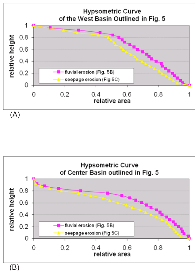
Figure 7. Hypsometric curve of the basin outlined in Figure 5 (the (a) west basin and (b) center basin).
