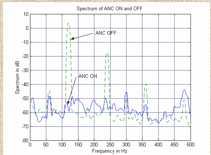
Performance of ANC system for vibratory bowl
