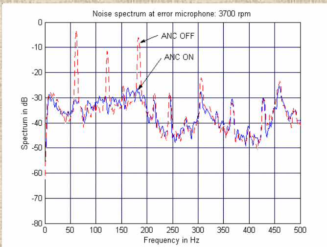
Performance of ANC system for the welding power generator
